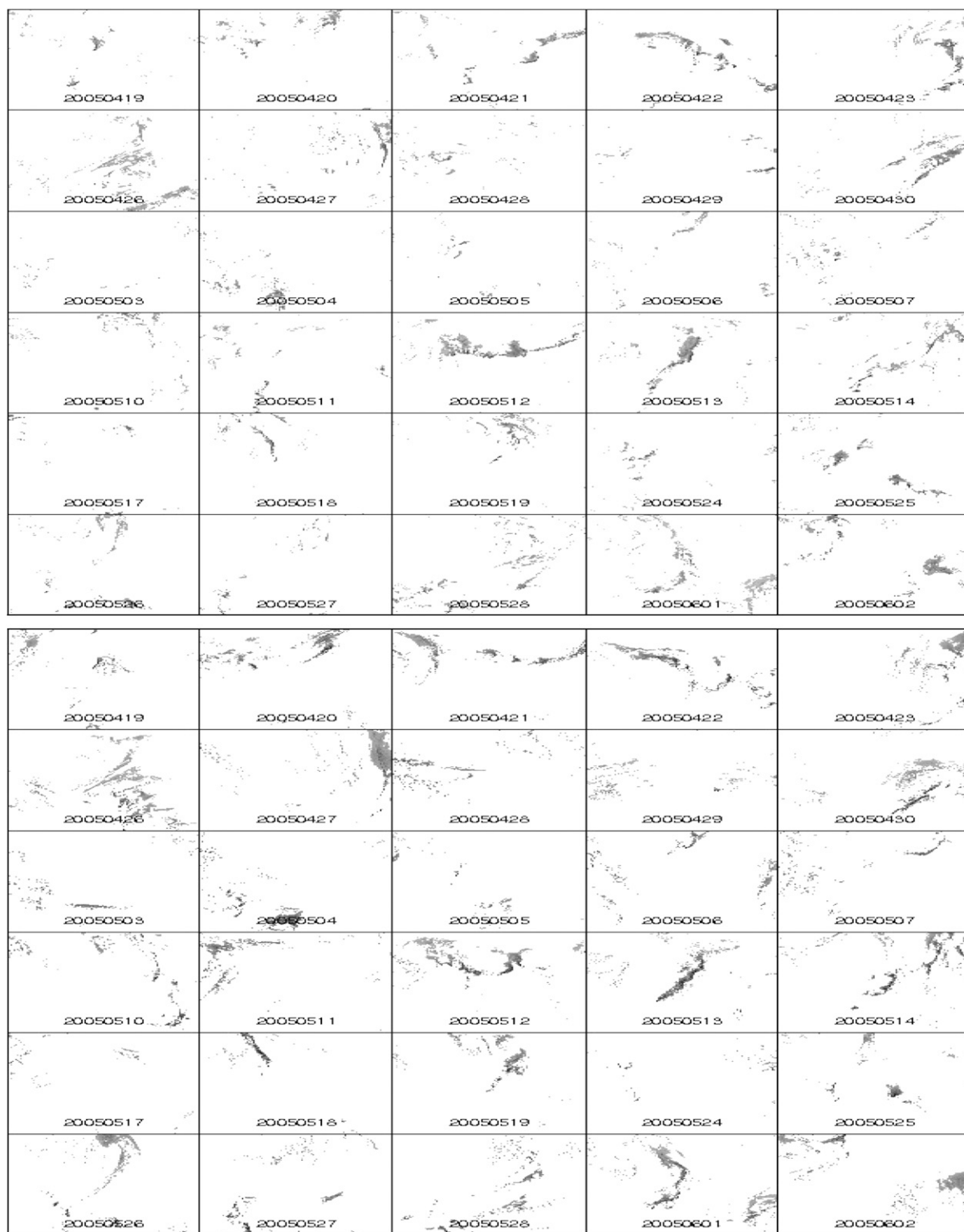
FIG. 2. (top) The 30 observation fields, with reflectivity exceeding 20 dBZ, examined here and (bottom) the corresponding arw2 forecasts.
