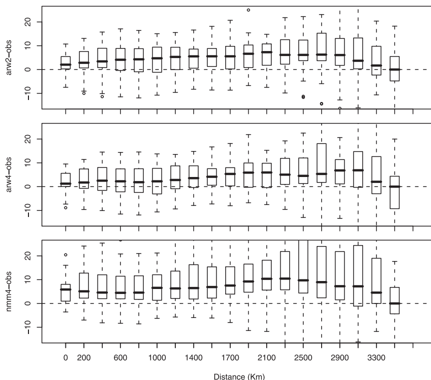
FIG. 8. The variation in the differences between variograms between days: (top to bottom) arw2 observation, arw4 observation, and nmm4 observation, respectively. The variograms are computed across the entire field.
