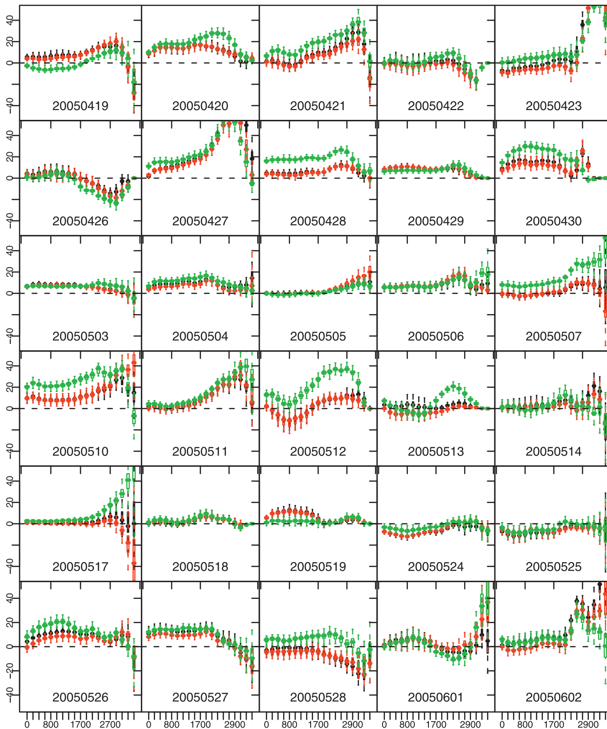
FIG. 7. The differences between variograms: arw2-observation (black), arw4 observation (red), and nmm4 observation (green).
