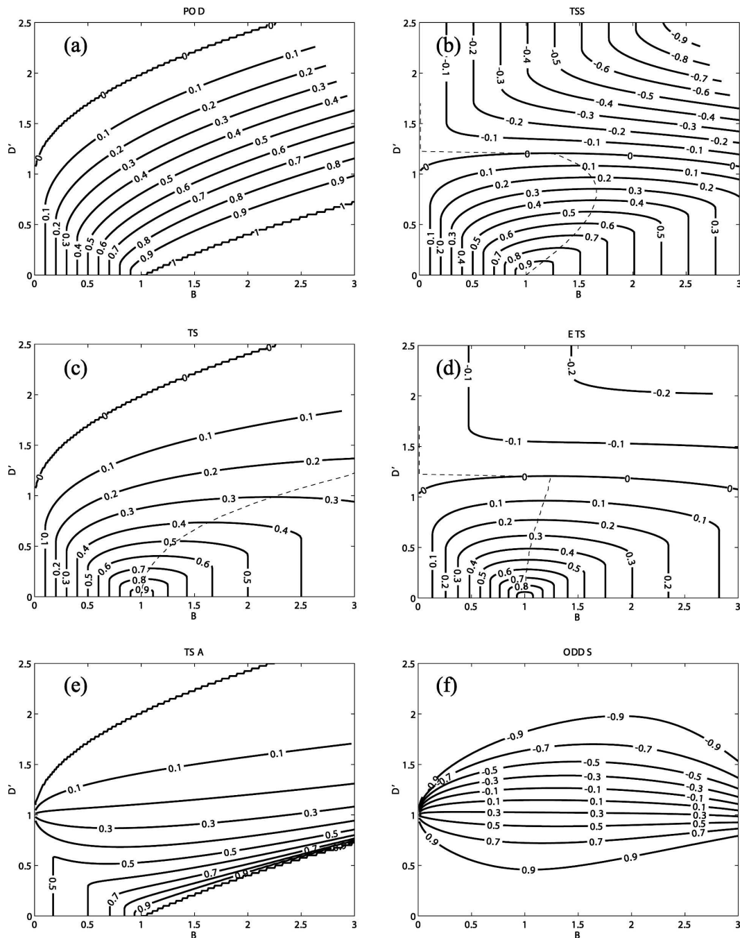
FIG. 3. As in Fig. 2 except for the relatively common event situation ( P \equiv 0.28 , observed circle radius r_o = 0.3 ).
