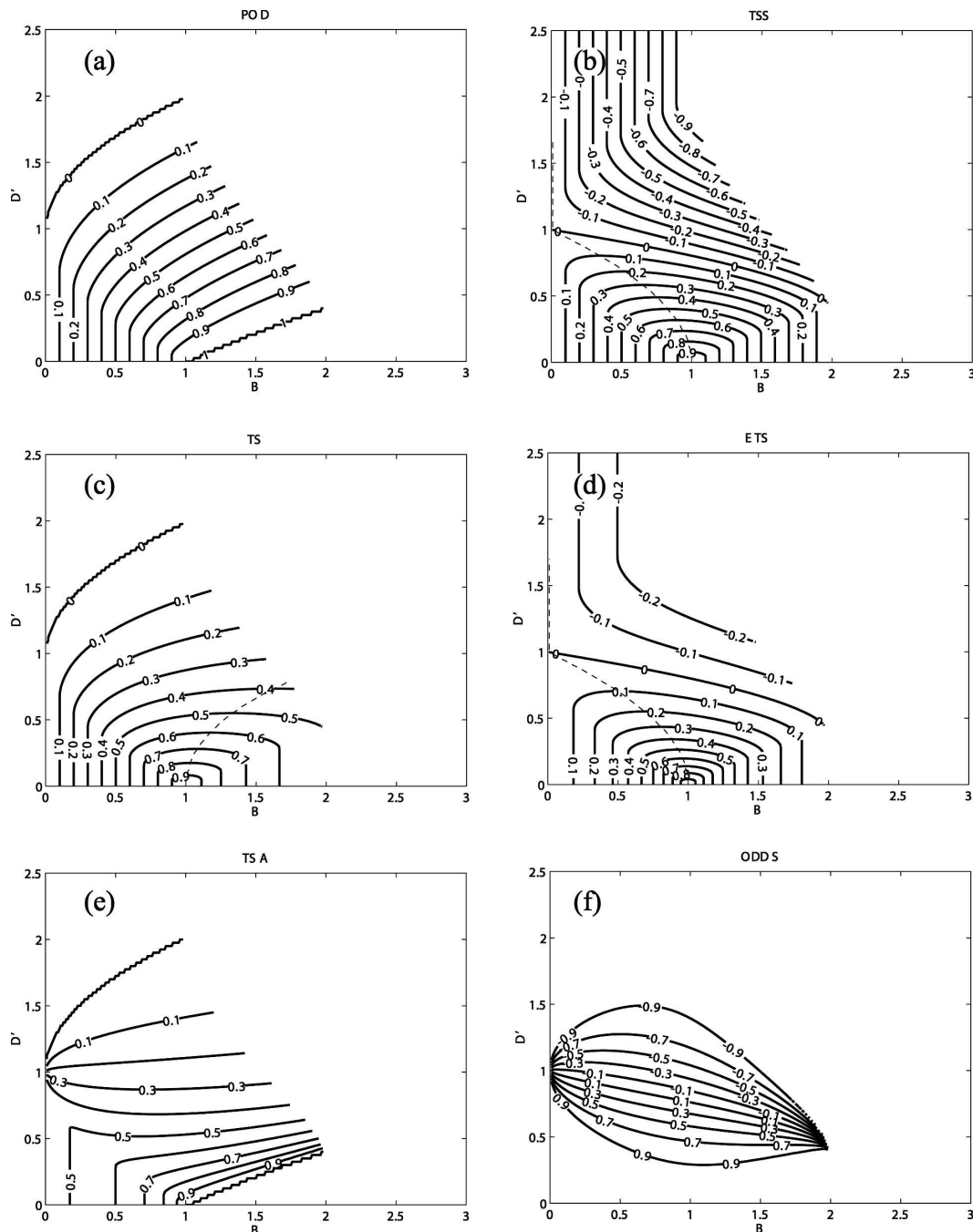
FIG. 5. As in Fig. 2 except for the very common event situation ( P \approx 0.50 , observed circle radius r_o = 0.4 ).
