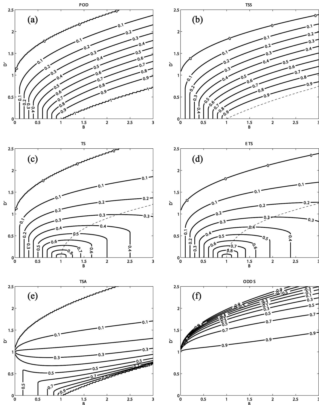
FIG. 2. For the rare event situation ( P \equiv 0.03 , observed circle radius r_o = 0.1 ), accuracy measures as a function of bias ( B ) and normalized displacement error ( D' ): (a) POD, (c) TS, and (e) TSA; (b) TSS, (d) ETS, and (f) ODDS. Axis of maximum score value is indicated in each plot by a dashed line. Contour interval is 0.1 in each panel except for ODDS, which uses a 0.2 contour interval.
